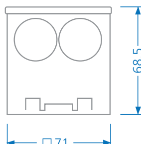
68,5'er installationsdåse
