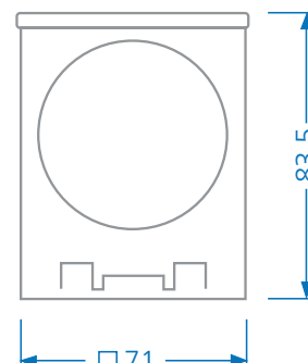
83,5'er installationsdåse
